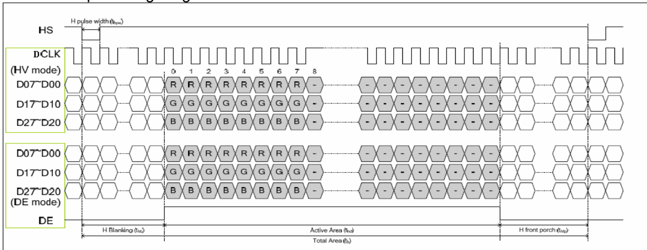
Horizontal input timing Diagram
